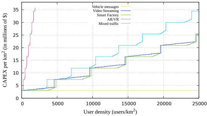
Fig. 13. Infrastructure CAPEX cost per \text{km}^2
