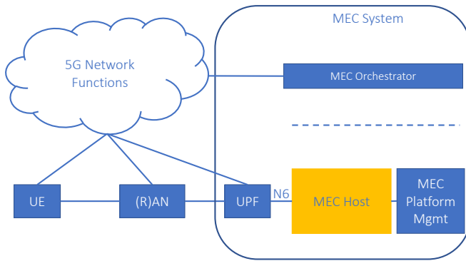
Fig. 6. MEC with 5G
