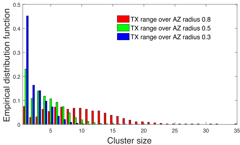
Fig. 9. Empirical distribution function of cluster size versus r/R for the industrial AZ in the Luxembourg scenario, for the low-density traffic period.
