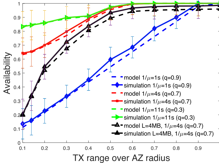
Fig. 3. Availability over transmission radius, with 95% confidence interval.
