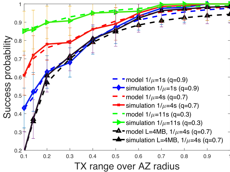
Fig. 2. Success probability over transmission radius, with 95% confidence intervals.
