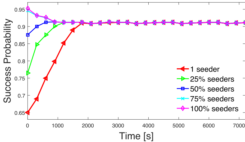
Fig. 7. Success Probability over simulation time. Several seeding strategies in the city center of Luxembourg City at high-density traffic (7AM – 9AM). Anchor Zone radius 260 m, transmission radius 160 m. At t = 0 there are 94 nodes within the AZ. Mean over sample population of 20 (each point) every 300 s.
