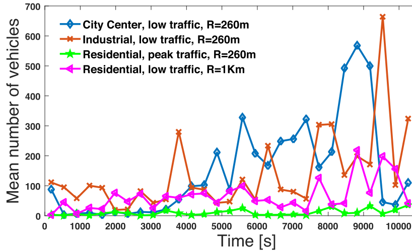
Fig. 11. Mean number of nodes in the three locations of the Luxembourg Scenario over simulation time.
