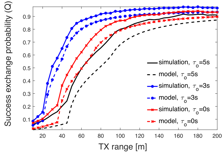
Fig. 4. Probability of successful content exchange Q vs transmission range, for three values of initial delay \tau_0 . Simulations are with a 95% confidence interval of 4%.
