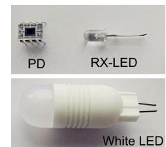
Fig. 5. Optical elements in our proposed system
