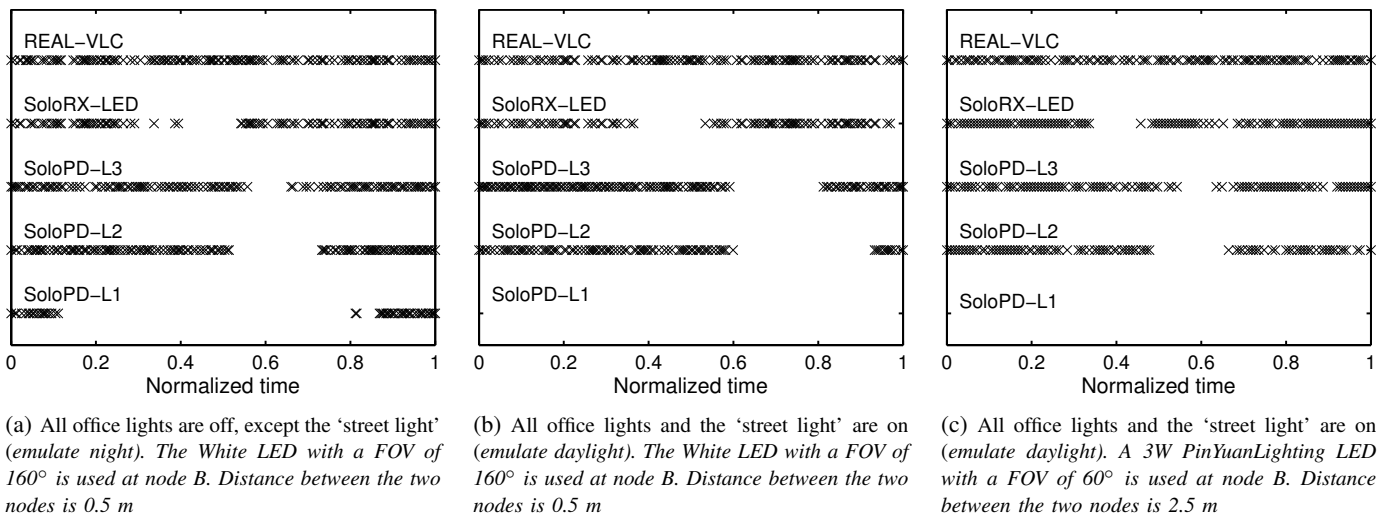
Fig. 19. Performance evaluation in a scaled down smart car application. Each marker ‘x’ represents the reception of one frame (payload is fixed to 200 bytes)
