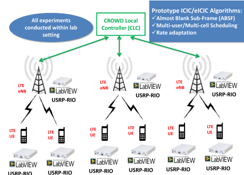
Fig. 8. LTE eICIC/ICIC Prototyping
