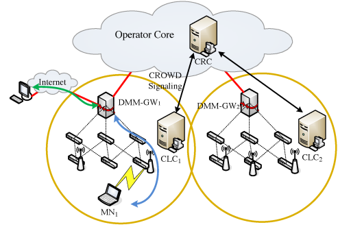
Fig. 5. SDN-based DMM architecture for mobility management.
