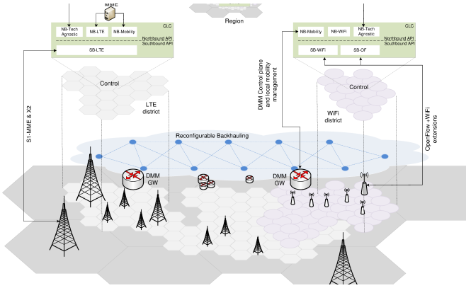
Fig. 1. CROWD architecture
