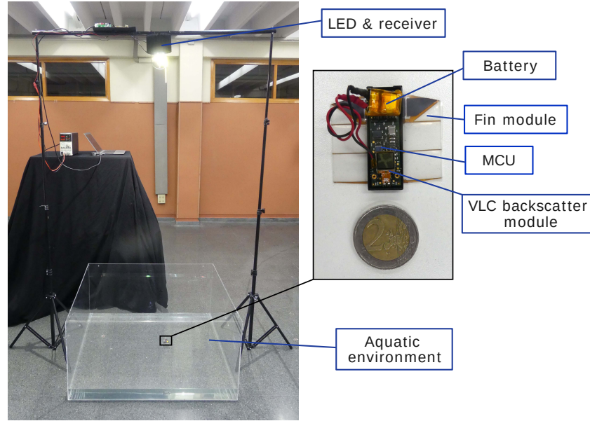
Fig. 18. Experimental setup for VLC backscatter communication for a swimming robot.
