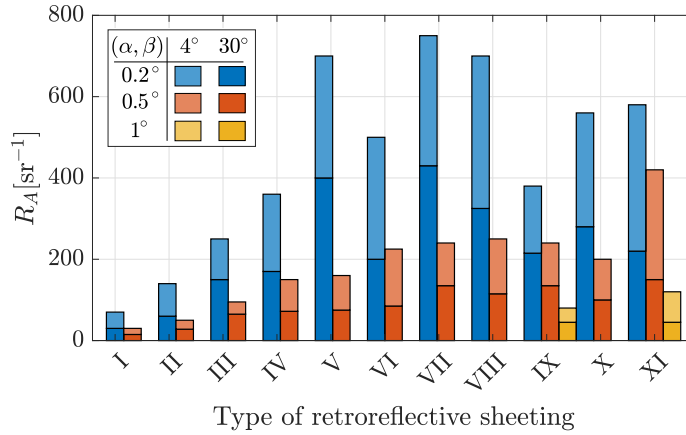
Fig. 10. R_A for different types of retroreflectors [5] for the reference values of \alpha (column) and \beta (row).
