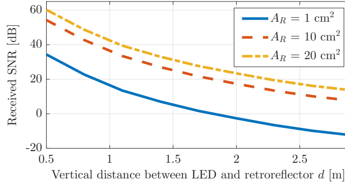
Fig. 11. Simulation of the received SNR versus vertical distance between LED-PD and retroreflector, for different retroreflector sizes ( A_R ) of Type XI and keeping all elements vertically aligned, i.e., \alpha = 0^\circ and \beta = 0^\circ .
