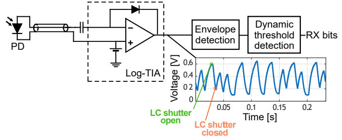
Fig. 15. VLC backscatter receiver circuit and analog received waveform.
