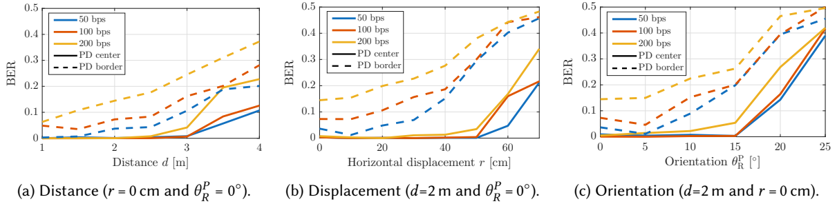
Fig. 16. BER of MiniRetro for different data rates and PD placements.
