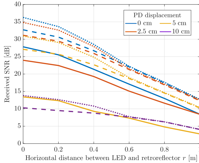
Fig. 12. Received SNR versus horizontal distance between LED/PD and retroreflector with A_R = 10 \text{ cm}^2 , keeping a vertical distance of 1 m, and for different PD displacements with respect to the LED center. Solid line: retroreflector Type VII. Dashed line: retroreflector Type IX. Dotted line: retroreflector Type XI.
