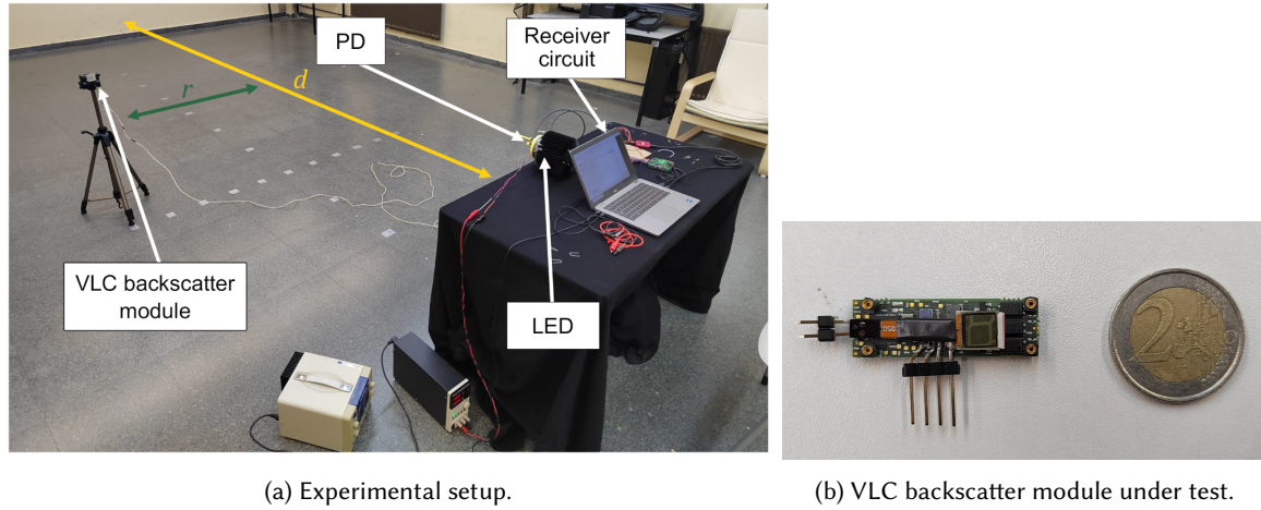
Fig. 13. Experimental setup and components used during the standalone evaluation.
