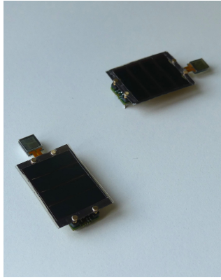
(a) Robot PCB with solar cells for optical downlink.
