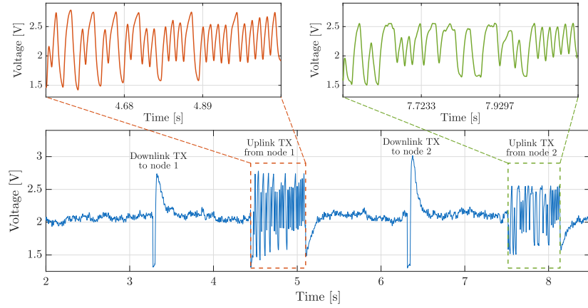
(b) Multiple node management through downlink VLC channel.
