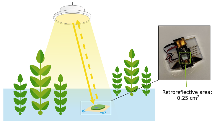
Fig. 1. Miniaturized VLC backscatter system for uplink in sustainable IoT use cases, such as aquaponics monitoring.
