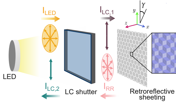
Fig. 7. Representation of how light travels through the LC shutter and retroreflector. We also represent how the modification of the light polarization is produced by the VLC backscatter module.
