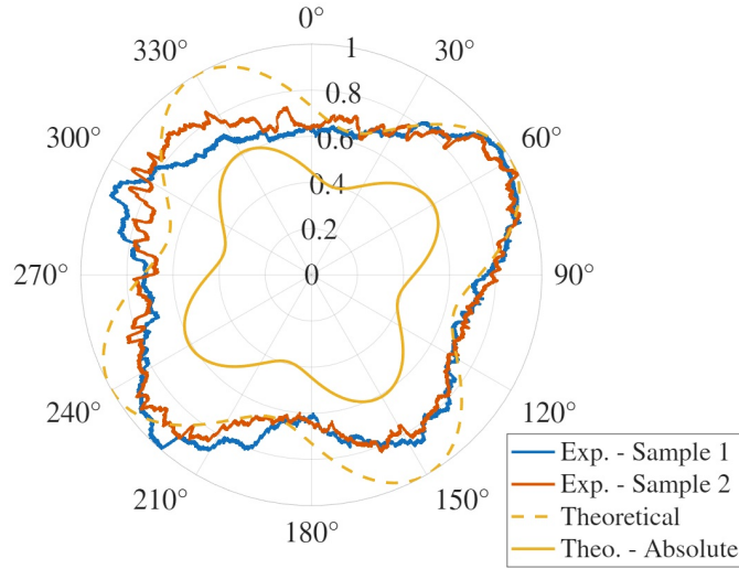
Fig. 9. Comparison of experimental and theoretical relative returned optical power from the VLC backscatter module with respect to angle \gamma .
