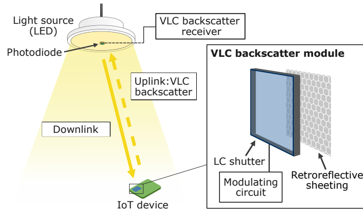
Fig. 2. Overview of the VLC backscatter system under study.
