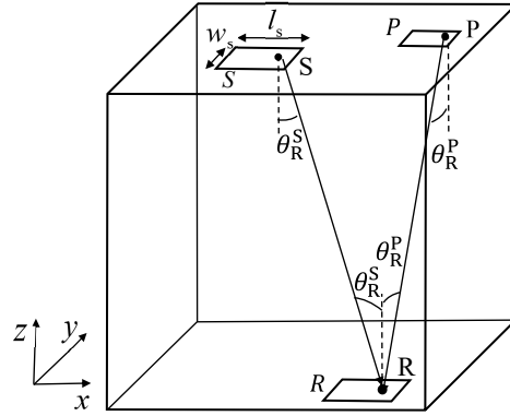
Fig. 4. System model including a light source (S), a retroreflector sheeting (R) and a photodetector (P).
