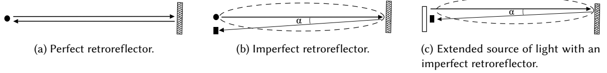
Fig. 5. Possible configurations of the three elements of the VLC backscatter link: light source, retroreflector and photodetector.
