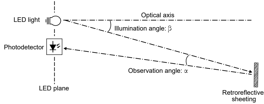
Fig. 6. Disposition of the LED, retroreflector and receiver in the VLC backscatter link, where angles \alpha and \beta determine R_A .
