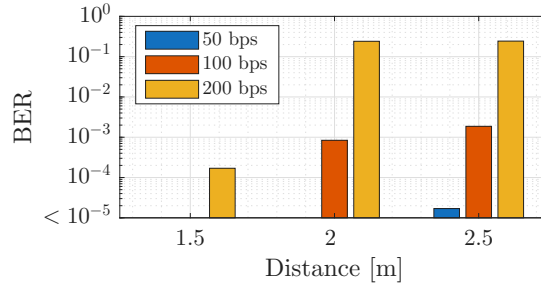
Fig. 19. BER for MiniRetro mounted on the swimming robot.
