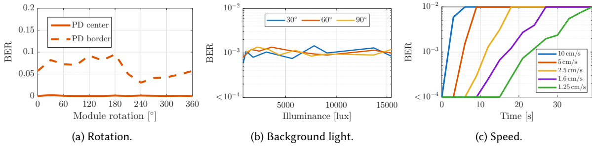
Fig. 17. Robustness of MiniRetro against rotation, background light, and movement ( d = 2 m, r = 0 cm and \theta_R^P = 0^\circ ).
