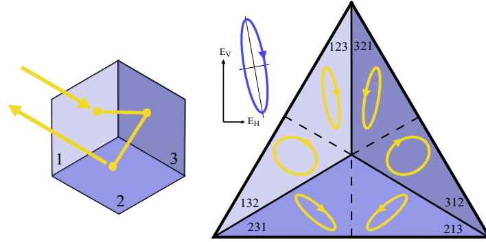
Fig. 8. Light reflection on a corner-cube retroreflector and output polarization for a vertically polarized input. This depends on the order in which light hits the three sides of the cube (left) and is determined by the first region abc onto which the light impinges (right).
