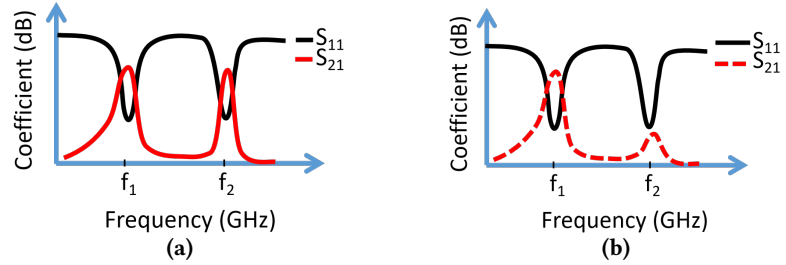
Figure 4: Return Loss Coefficient ( S_{11} ) and Mutual Coupling coefficient ( S_{21} ) of two antennas (a) without, and (b) with antenna location optimization. By optimizing the mutual coupling of the antennas, mmPlug ensures that the LNA and loop resonate only at f_1 .
