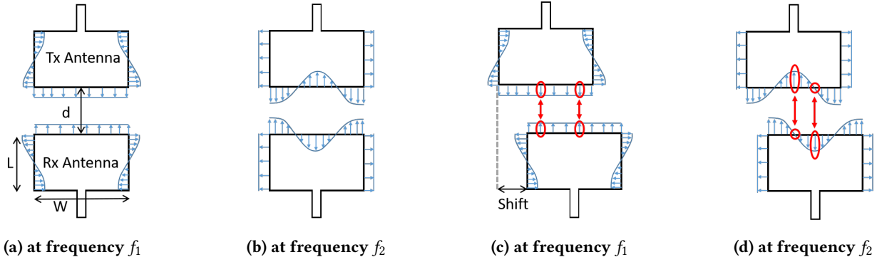
Figure 5: Patch Antenna's electric field at different operating frequencies and antennas arrangement. Patch antennas typically have two resonate frequency ( f_1 and f_2 ) which are determined by by L and \frac{W}{2} , respectively. At f_1 , the facing edges of the two antennas have uniform fields, and hence any shift in the antennas positions will not impact on the coupling at that frequency (see a and c). However, at f_2 , the facing edges of the two antennas have sinusoidal field, and hence a shift will significantly reduce the coupling at that frequency since the peaks and nodes of the field do not match anymore (see b and d).
