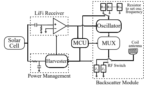
Figure 7: Block diagram of LeakageScatter battery-free tag.
