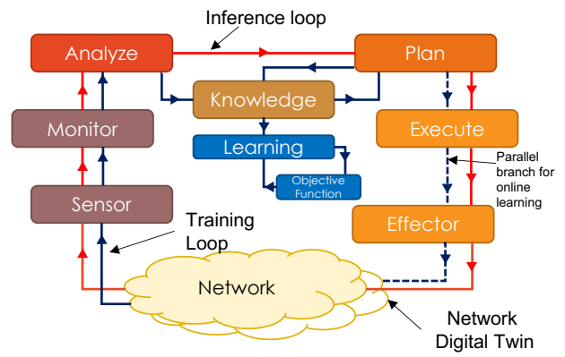
Fig. 3: Extended N-MAPE-K abstractions for NI algorithms
