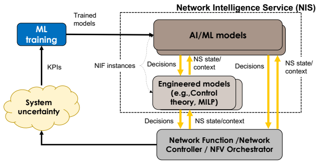
Fig. 2: Taxonomy of NIP operations
