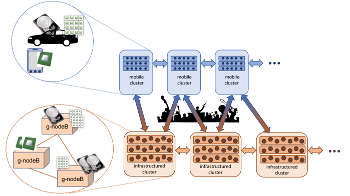
Figure 2. V-Edge architecture: Logical resources from mobile users and infrastructure-based systems (e.g., edge servers co-located with a gNB) are aggregated into clusters. Multiple clusters are appropriately coordinated and microservices can migrate from one cluster to another to optimize the service location. Resource management is done by an orchestrator, which may interwork with others, controlling neighboring clusters, to migrate services.
