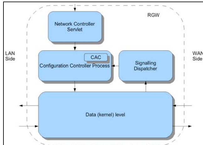
Fig. 4. RGW management architecture
