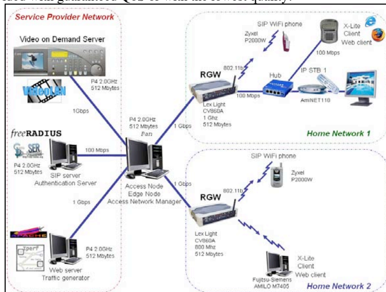
Fig. 6. Network trial testbed
