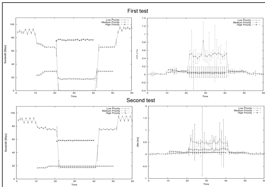
Fig. 7. Bandwidth and jitter value for the first and the second test
