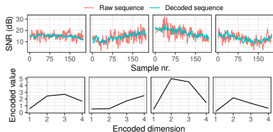
Fig. 14. Examples of 200-dimensional raw vs reconstructed SNR sequences (top). 4-dimensional encoded representations (bottom).
