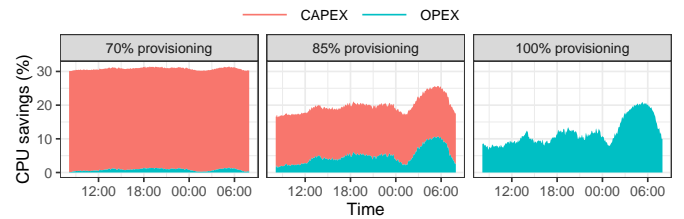
Fig. 26. vrAIn’s savings relative to a static computing-agnostic approach provisioned with sufficient CPU resources for the peak demand.
