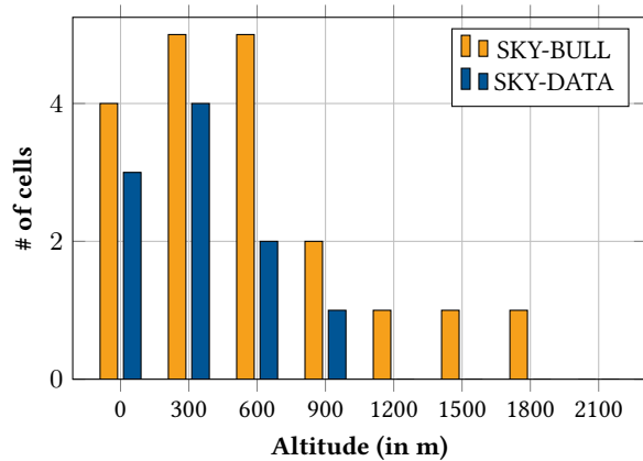
Figure 12: Number of LTE cells detected at different altitudes.
