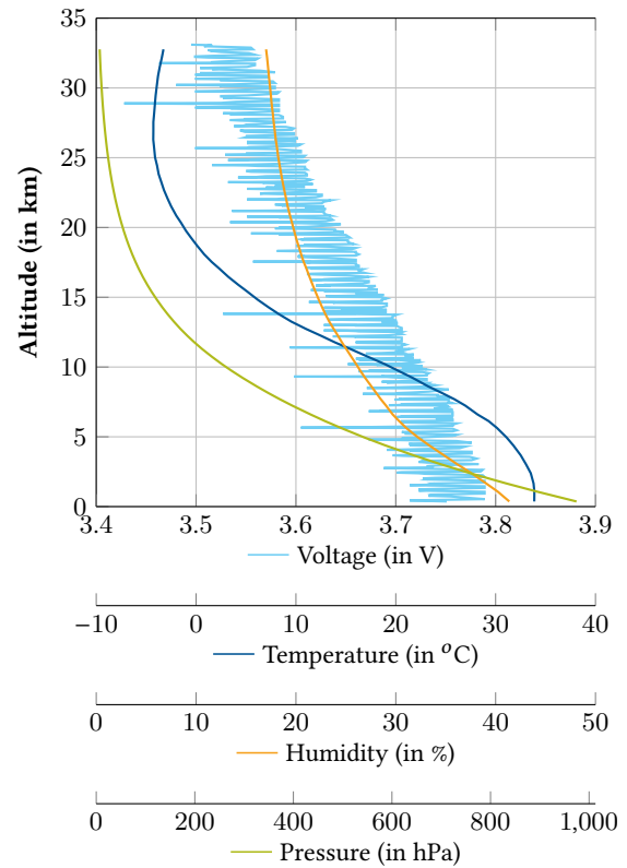
Figure 5: Typical measurement results of the on-board flight computer in one of the flights.
