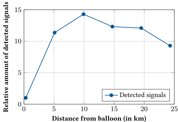
Figure 15: Relative amount of detected signals in the 434.5 MHz band.
