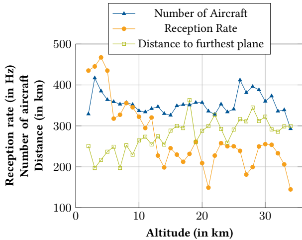
Figure 7: Amount of aircrafts picked up by the balloon at various altitudes compared to the reception rate of ADS-B messages.
