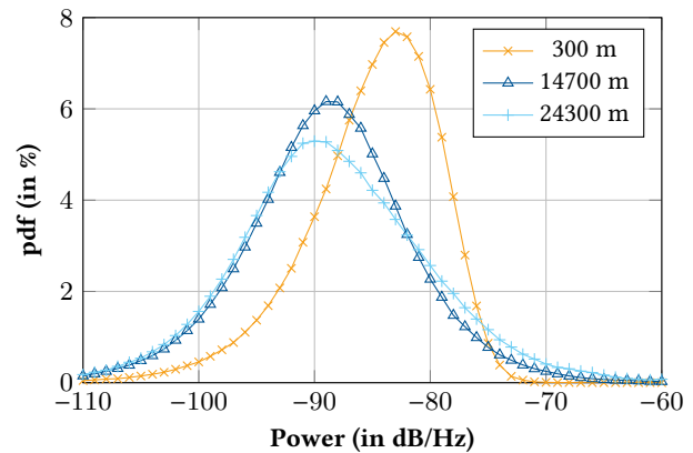
Figure 13: Probability density function of combined noise and signal PSD values for three different altitudes.
