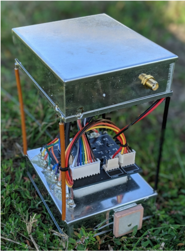
Figure 1: Balloon payload encompassing all the hardware required for spectrum measurements in the stratosphere.
