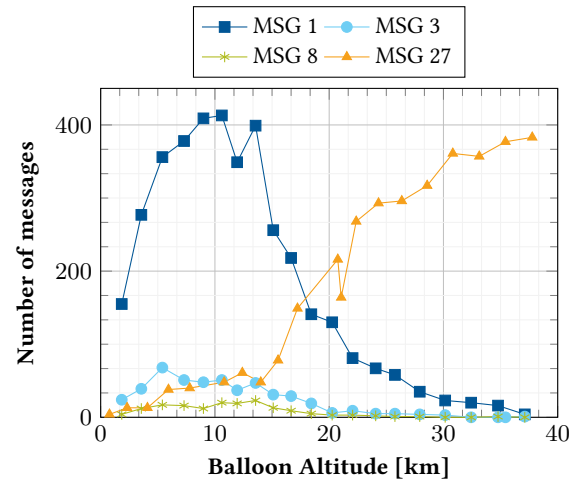
Figure 10: AIS Message Types Occurrence Frequency.
