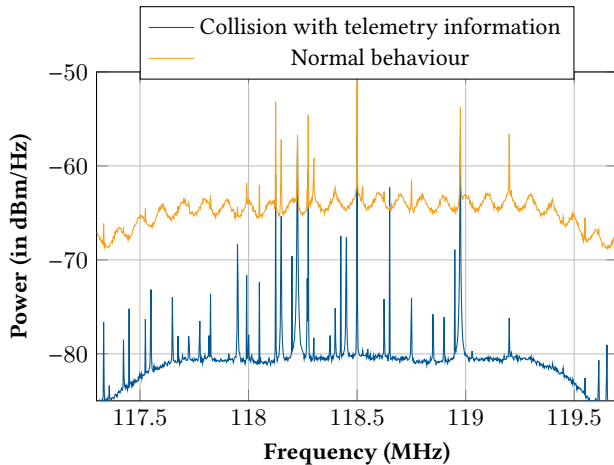
Figure 16: Power loss in the received signal for ATC traffic.
