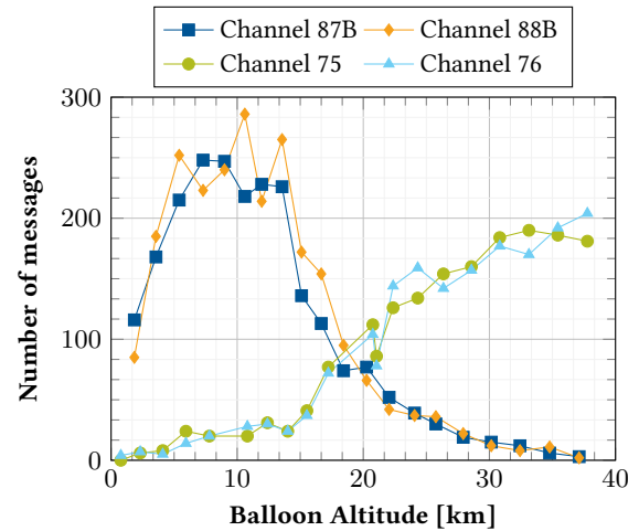
Figure 11: Number of AIS Messages per channel.
