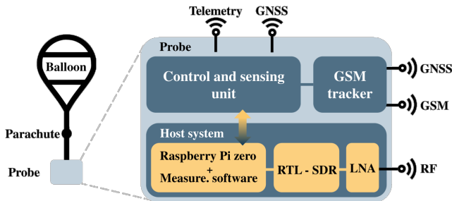
Figure 3: Hardware design of the probe, consisting of the FRCU, a Raspberry Pi Zero W, an RTL-SDR along with a LNA
