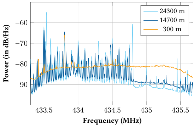
Figure 14: PSD for three different altitudes.
