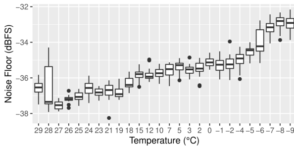
Figure 8: Noise level of the ADS-B messages in the balloon.
