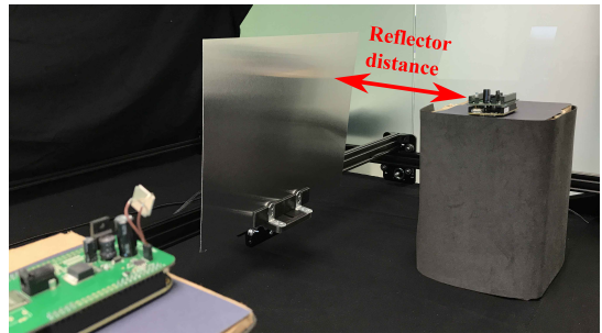
Fig. 2: Testbed.
