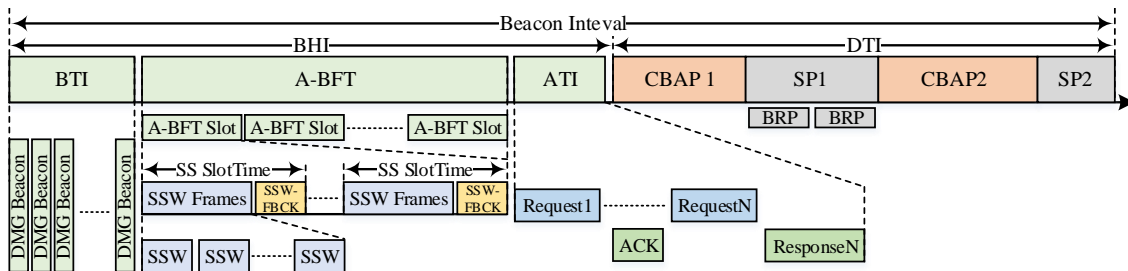
Figure 2.2: IEEE 802.11ad beacon interval with different access periods.
