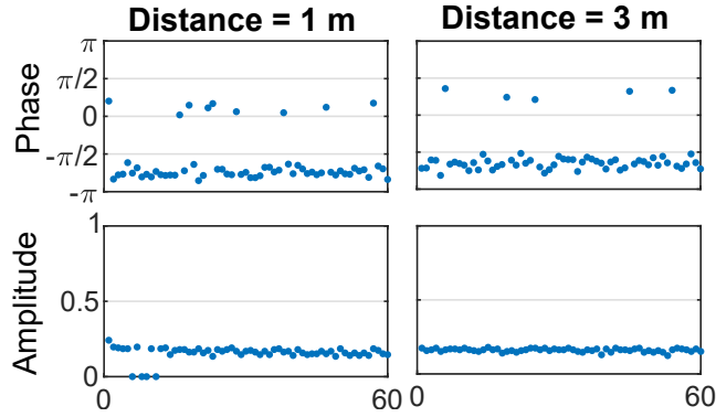
Figure 7.5: CSI Measurements vs Distance.
