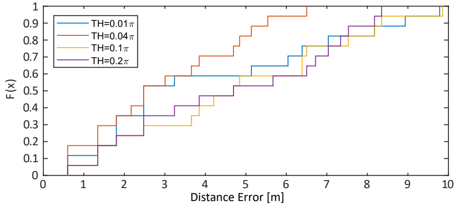
Figure 7.10: Empirical CDF.
