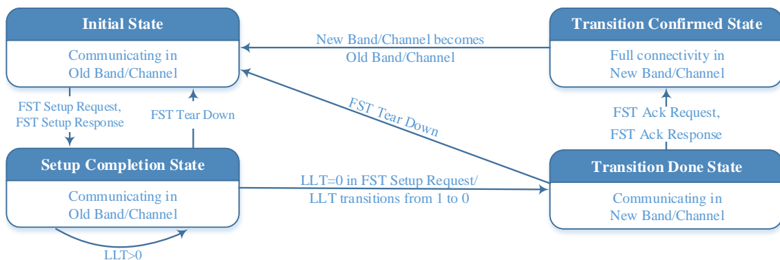
Figure 3.11: FST state machine.
