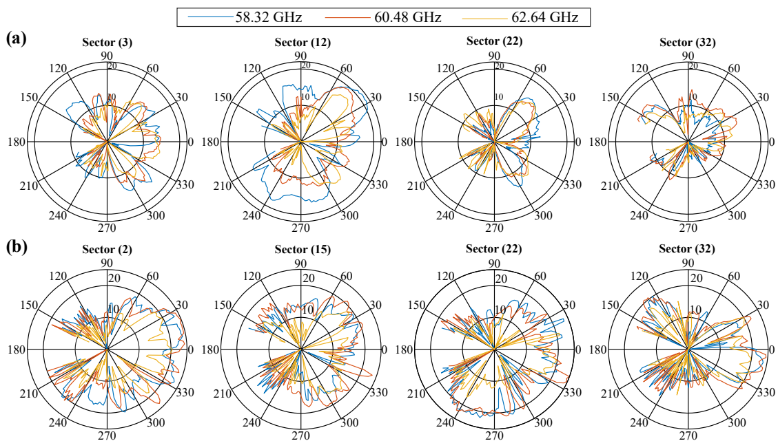
Figure 6.15: Beam Patterns Comparison for Different Frequency Channels (a) Beam Patterns for the TALON Router (b) Beam Patterns for MikroTik Router.
