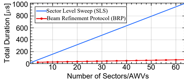
Figure 4.8: Beamforming Duration for BRP and SLS
