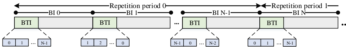
Figure 3.8: DMG Beacon transmission by PCP/AP during the BTI [1].
