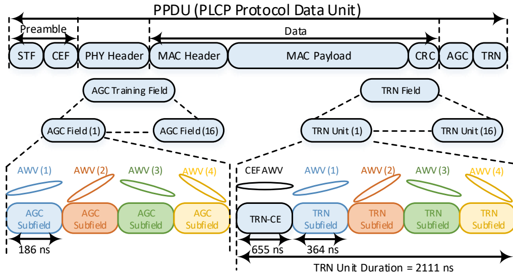
Figure 3.2: DMG Frame Structure with AGC and TRN Subfields for BRP-TX Packet.
