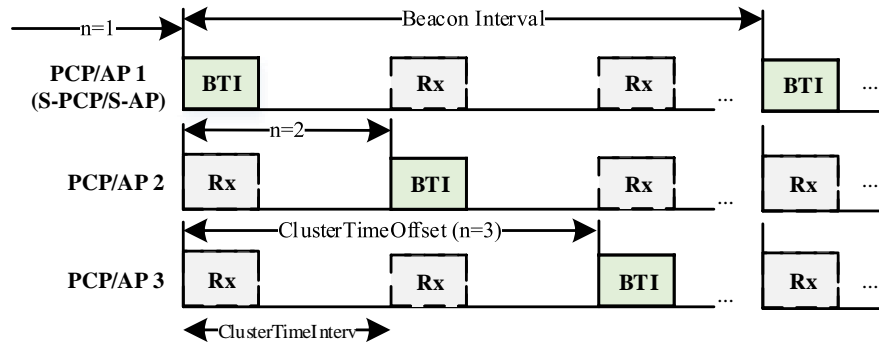
Figure 3.15: Decentralized Clustering for 3 PCPs/APs [1].
