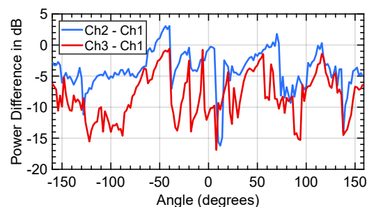
Figure 6.16: Antenna Array Directivity Difference with Respect to the Lowest Channel
