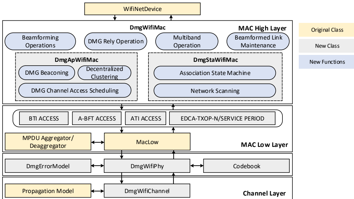
Figure 3.1: IEEE 802.11 architecture in ns-3 with 802.11ad Features.
