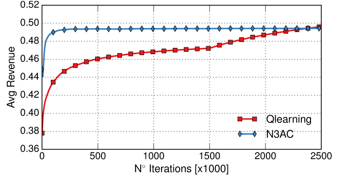
Fig. 6: Learning time for N3AC and Q-learning.
