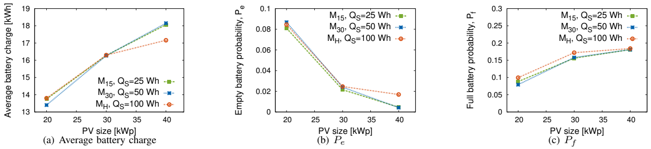
Fig. 15. Average battery charge, empty ( P_e ) and full ( P_f ) battery probabilities versus PV panel sizes, for different time slots, for Turin with N_W = 5 and equal-range discretization, for C_B = 25 kWh, with residential weekday traffic profile, adopting the Earth model.
