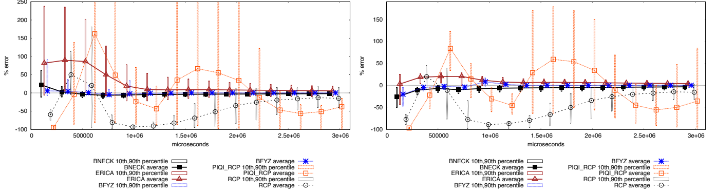
Figure 10: Experiment 2a. Error distribution at sources (left) and bottlenecks (right).
