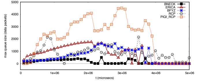
Figure 11: Experiment 2b. Maximum queue sizes.
