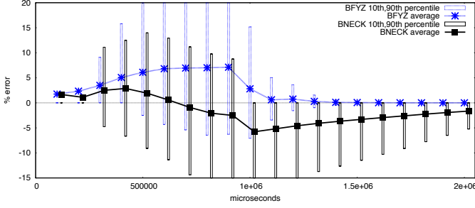
Figure 12: Experiment 2c. Error distribution at (left) sources and (right) bottlenecks.
