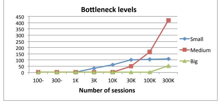
Figure 7: Average bottleneck levels observed in Experiment 1 with different network topologies.
