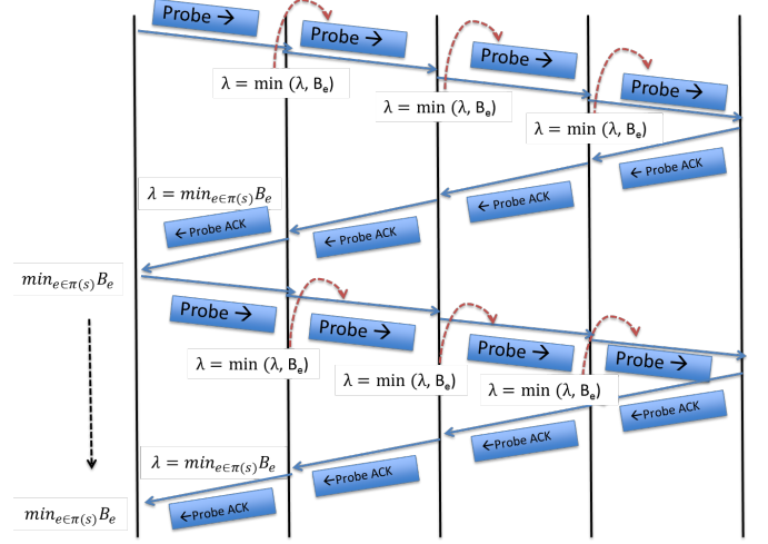
Figure 3: EERC protocol.
