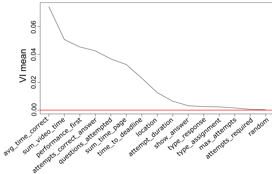
Figure 6.4: Descendent ranking of variables in terms of VI.
