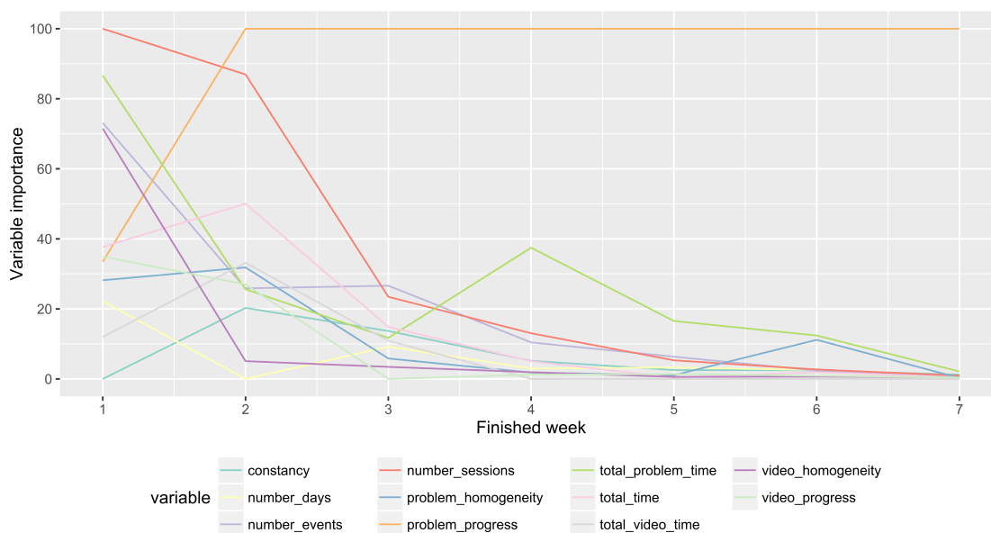
Figure 6.3: Evolution of variable importance of the GBM model in each week.
