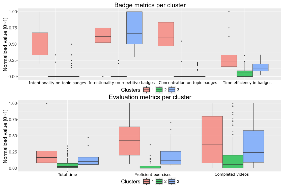
Figure 5.4: Boxplot visualization of the indicators separated by cluster. The upper plot shows the badge metrics and the bottom plot the evaluation fields.
