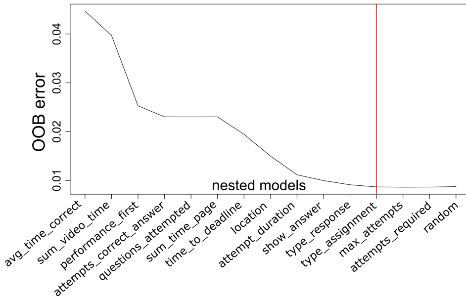
Figure 6.5: Nested collection of random forest models.
