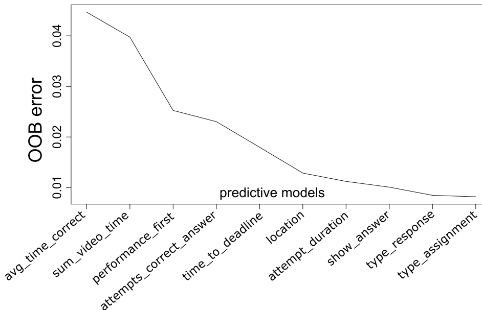
Figure 6.6: Sequence of RF models constructed using a stepwise procedure.
