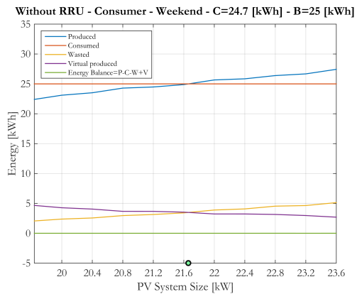
Fig. 17. Energy balance vs PV panel size; C = 24.7 kWh and B = 25 kWh.
