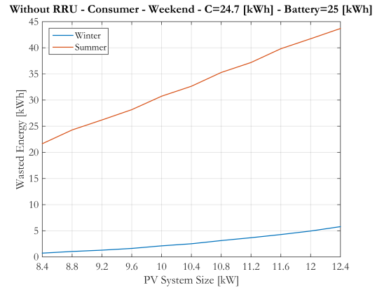
Fig. 13. Wasted energy vs PV panel's size in winter and summer when C = 24.7 kWh and the battery capacity is B = 25 kWh.
