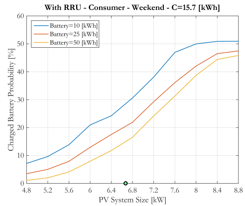
Fig. 4. Charged battery probability vs PV panel's size for several battery capacities when C = 15.7 kWh.
