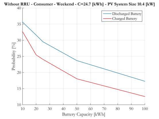
Fig. 9. Discharged and charged battery probability vs battery capacity when C = 24.7 kWh and the PV panel's size is 10.4 kW.
