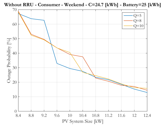
Fig. 14. Outage probability vs PV panel's size for different quantization levels of irradiance when C = 24.7 kWh and the battery capacity is B = 25 kWh.
