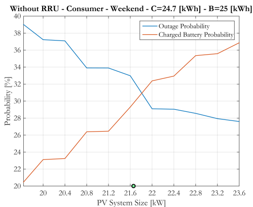
Fig. 16. Discharged and charged battery probabilities vs PV panel size; C = 24.7 kWh and B = 25 kWh.
