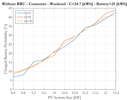
Fig. 15. Charged battery probability vs PV panel's size for different quantization levels of irradiance; C = 24.7 kWh and B = 25 kWh.
