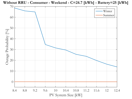
Fig. 12. Outage probability vs PV panel's size in winter and summer when C = 24.7 kWh and the battery capacity is B = 25 kWh.
