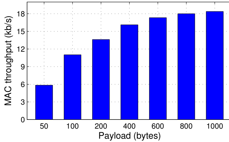
Figure 2.4: MAC layer throughput as a function of the per-frame payload.
