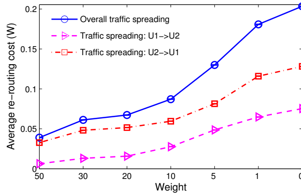
Figure 5.8: Average re-routing rate of each user under greedy scheduler where \lambda = \{0.19, 0.21\} arrivals/sec and \mathbf{d} = \{92, 100\} m.
