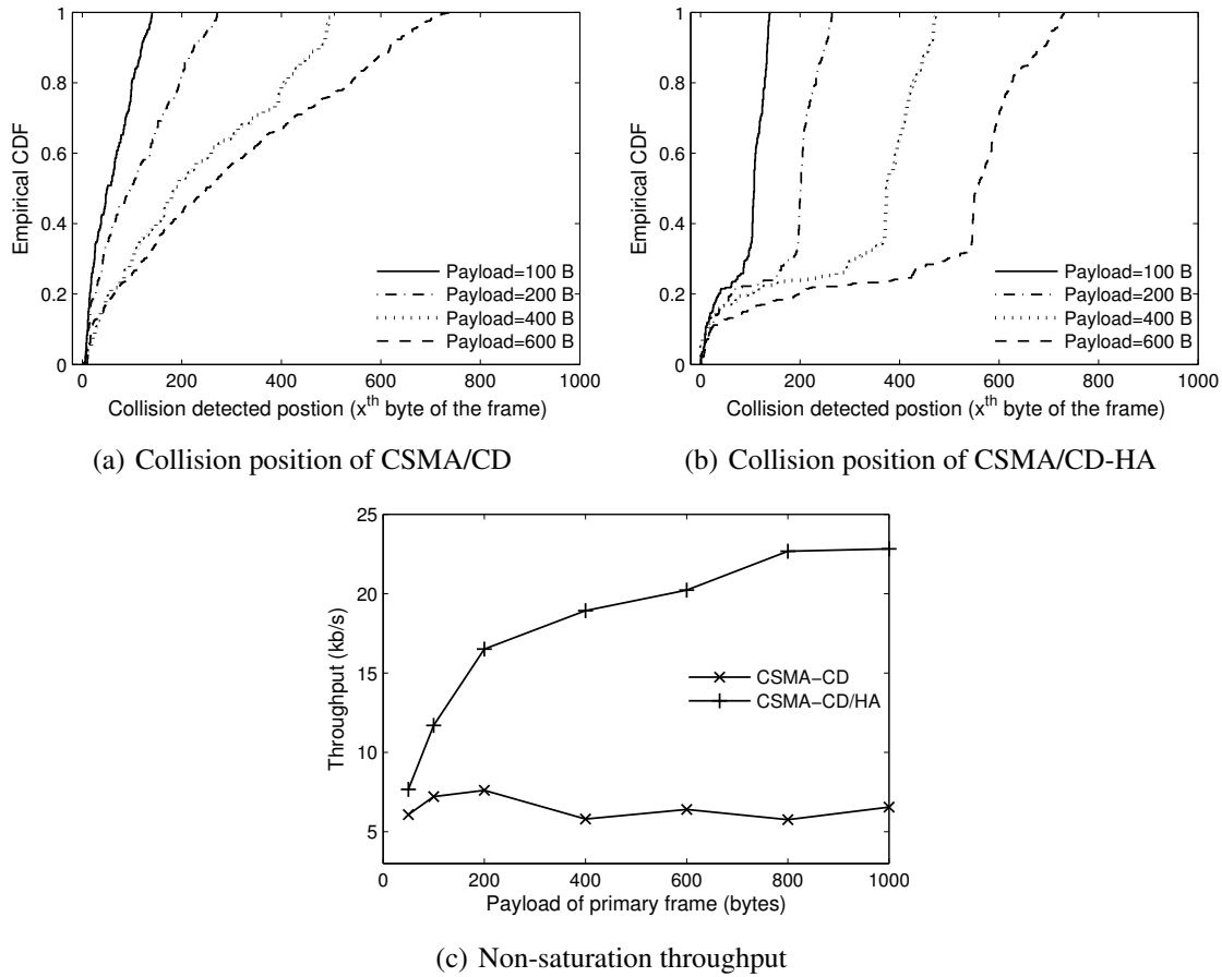
Figure 3.13: Evaluation results of the three-node network with hidden nodes.
