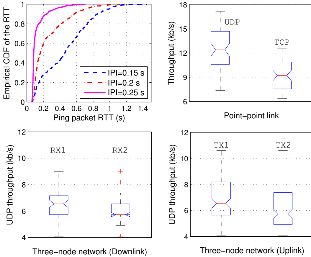
Figure 2.5: System-level evaluation results using ping and iperf.
