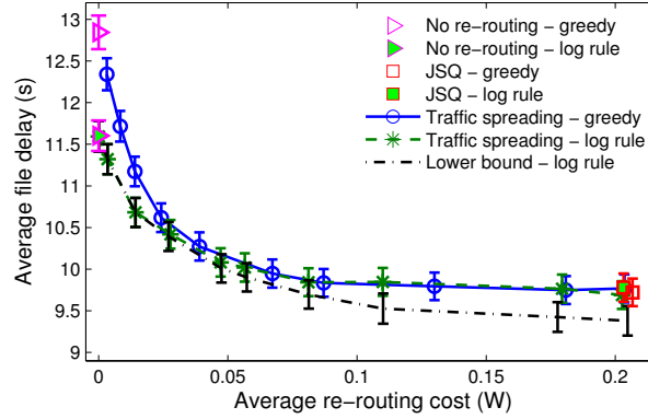
Figure 5.7: Performance vs. re-routing cost under two-user heterogeneous scenarios where \lambda = \{0.19, 0.21\} arrivals/sec and \mathbf{d} = \{92, 100\} m.
