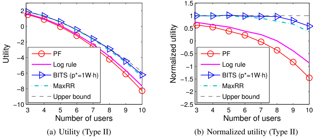
Figure 6.8: Homogeneous scenarios with different number of users: the average \text{SNR}^{\text{bs-user}} = \{9, 9\} dB, \text{SNR}_{ij}^{\text{user-user}} = 9 dB, i \neq j .
