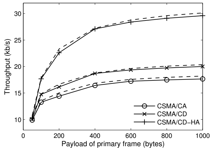
Figure 3.12: Evaluation results of a three-node network ( corresponding analytical results are represented by the dash lines ).
