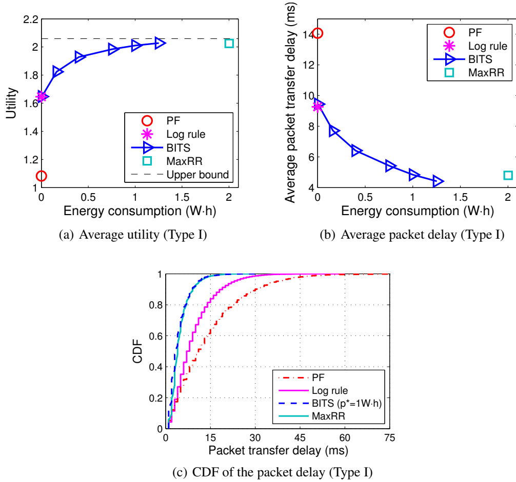
Figure 6.5: Two-user homogeneous scenario: the average \text{SNR}^{\text{bs-user}} = \{9, 9\}\text{dB} , \text{SNR}_{ij}^{\text{user-user}} = 9\text{dB} , \lambda = \{2, 2\}\text{packets/ms} , i \neq j .
