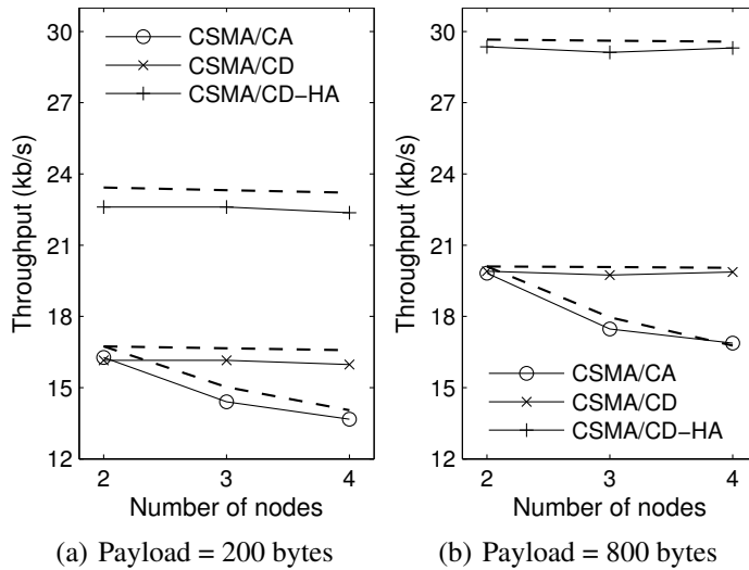
Figure 3.11: Evaluation results of an ad-hoc network with different payloads of primary frames and different number of nodes ( corresponding analytical results are represented by the dash lines ).
