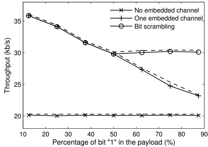
Figure 3.14: Evaluation results of a point-to-point link with bit scrambling ( corresponding analytical results are represented by the dash lines ).
