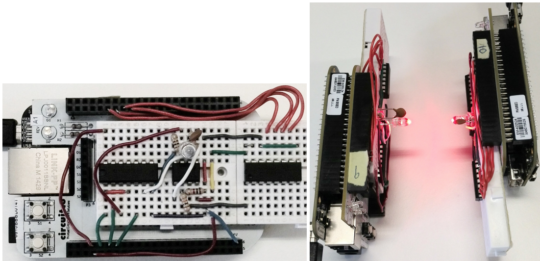
Figure 2.1: The initial prototype of OpenVLC: the front-end transceiver of an OpenVLC node is shown on the left, and an example of inter-node communication is shown on the right.
