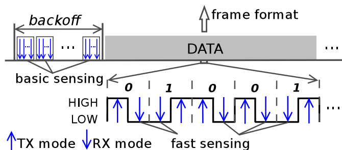
Figure 2.3: Backoff, basic and fast sensing of the CSMA/CD protocol. The transmitter uses OOK with Manchester coding to send data. In the frame format: Length > 0 \iff DATA; Length = 0 \iff ACK.
