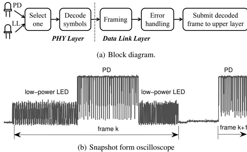
Figure 4.17: The system can decide which receiver antenna to use (switch the RX between the LL and PD) at anytime
