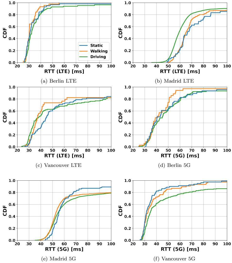
Figure 9: RTT Comparison across different mobility modes (Static: blue, Walking: orange, Driving: green).
