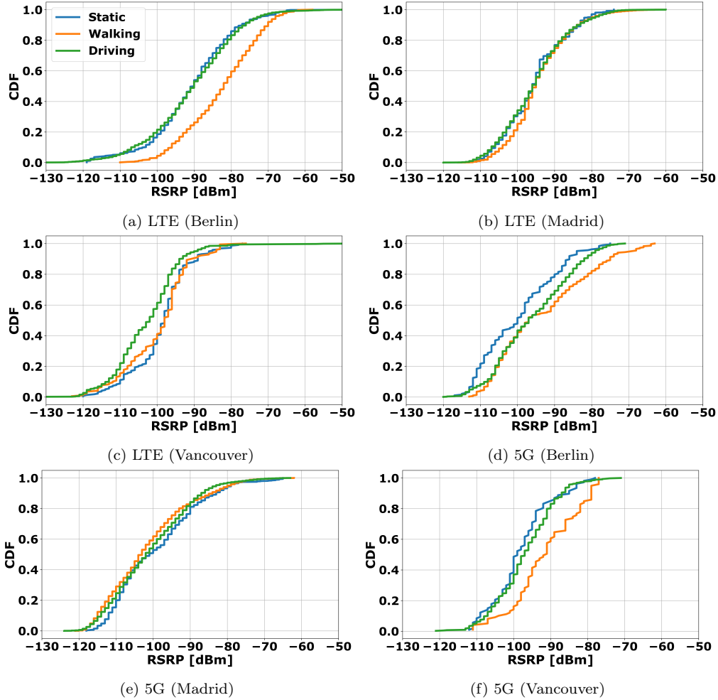
Figure 10: RSRP comparison across different mobility modes (Static: blue, Walking: orange, Driving: green).
