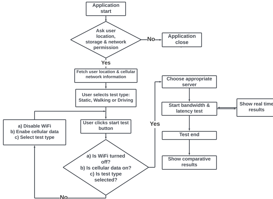
Figure 1: Workflow of the NextG-UP application.
