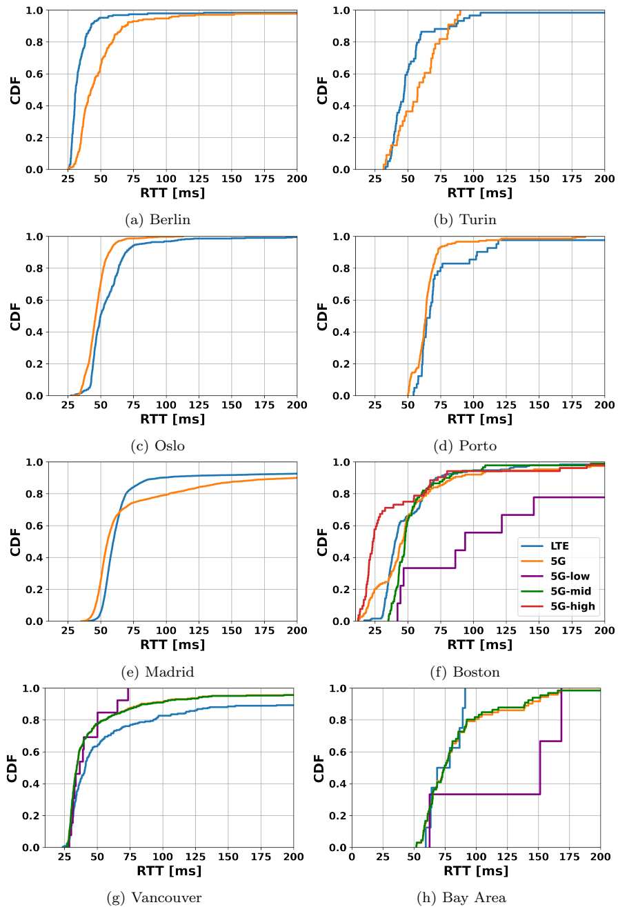
Figure 6: Latency comparison across different cities. LTE: blue, 5G (5G-low/mid/high combined): orange, 5G-low: purple, 5G-mid: green, 5G-high: red. Not all 5G bands are available in every North American city. For instance, Vancouver lacks mmWave base stations, and T-Mobile in the Bay Area does not offer 5G mmWave service.
