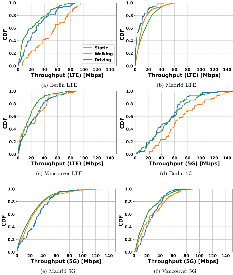
Figure 8: Throughput Comparison across different mobility modes (Static: blue, Walking: orange, Driving: green).
