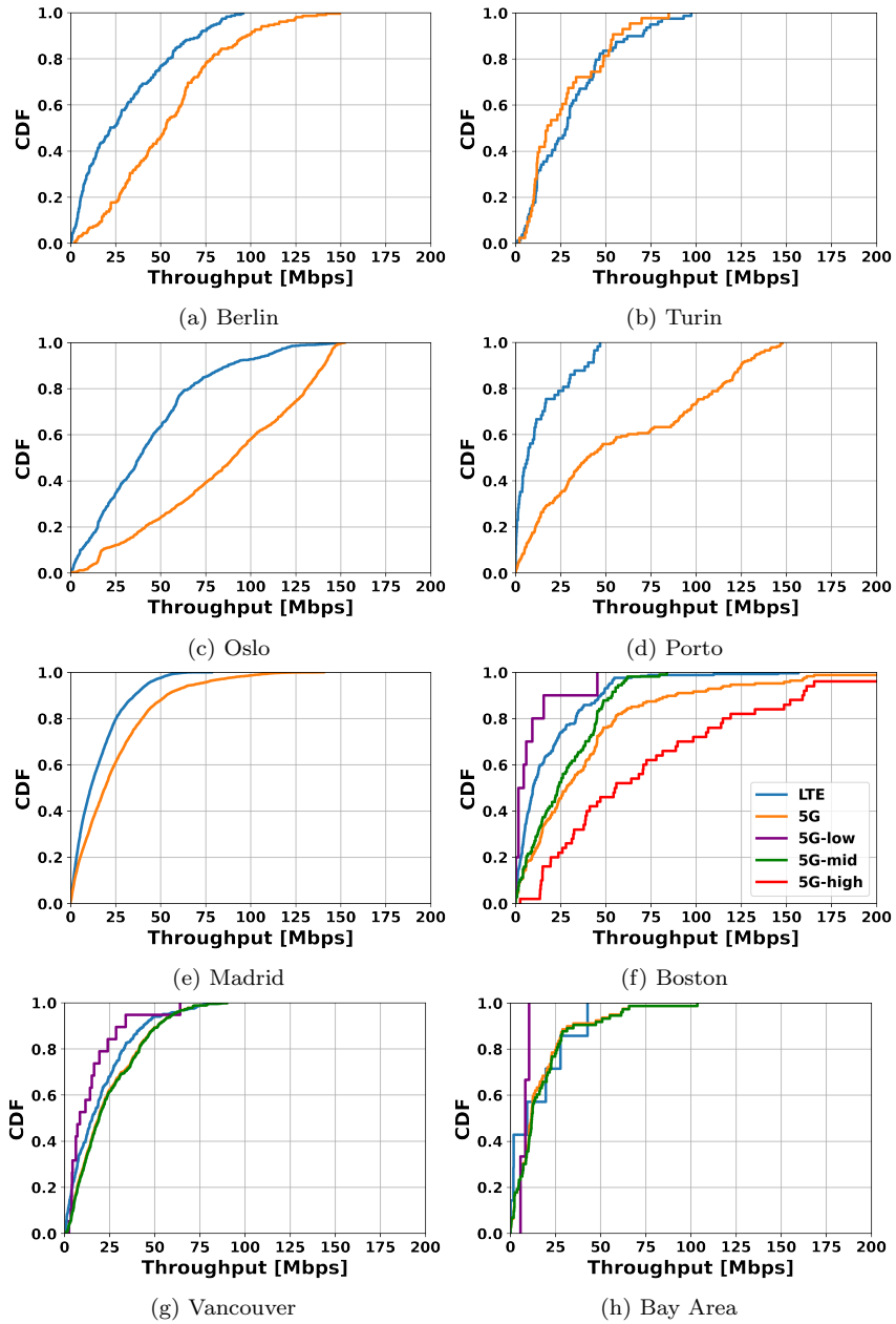
Figure 5: Throughput comparison across different cities. LTE: blue, 5G (5G-low/mid/high combined): orange, 5G-low: purple, 5G-mid: green, 5G-high: red. Not all 5G bands are available in every North American city. For instance, Vancouver lacks mmWave (5G-high) base stations, and T-Mobile in the Bay Area does not offer 5G mmWave service.
