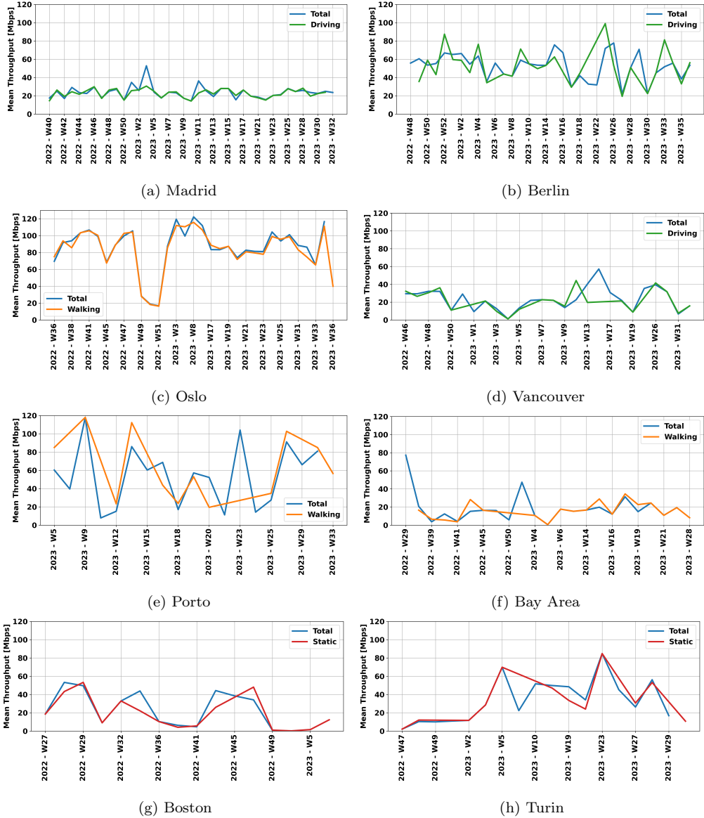
Figure 3: Evolution of 5G in terms of throughput. Throughput samples collected over a week are averaged and the average throughput over each week is plotted as a timeline. Blue represents the total samples collected by static, walking, and driving measurements combined. Red represents static, orange represents walking, and green represents driving samples only.
