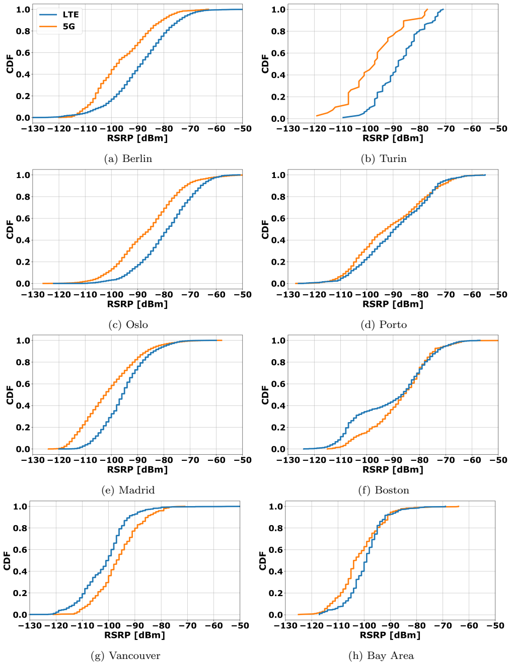
Figure 7: RSRP comparison across different cities (LTE: blue, 5G: orange).
