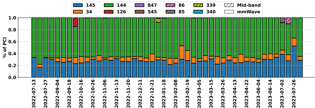
Figure 19: 5G PCI distribution during mobility. Hatched '///' bars represent 5G-midband PCIs. Clear bars represent 5G-mmWave PCIs.
