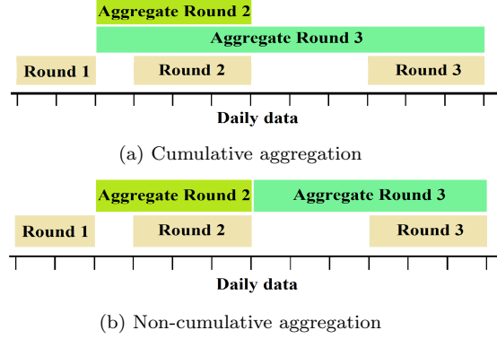
Figure 2: Diagrams showing how daily data points are aggregated to transform daily data into sporadic data.
