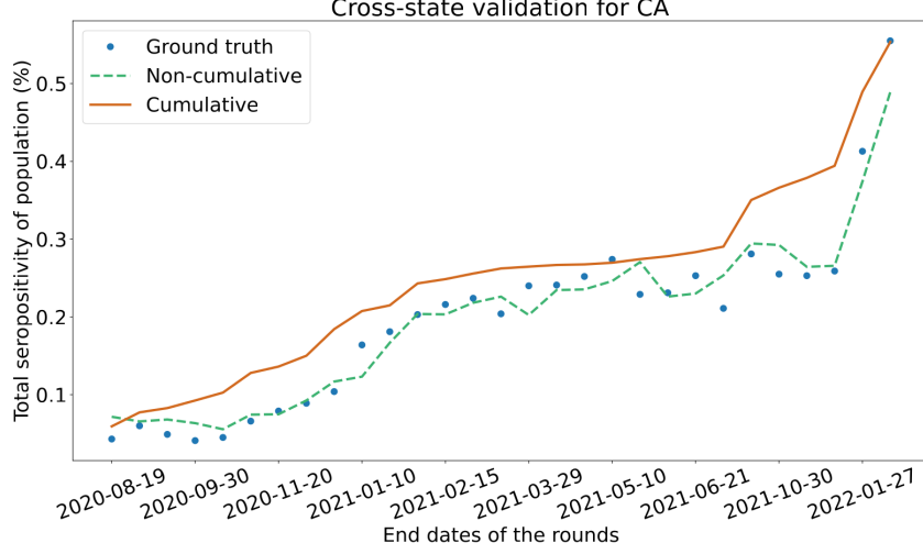
Figure 13: LR cross-state validation of California (CA) using the other ten most populous states.
