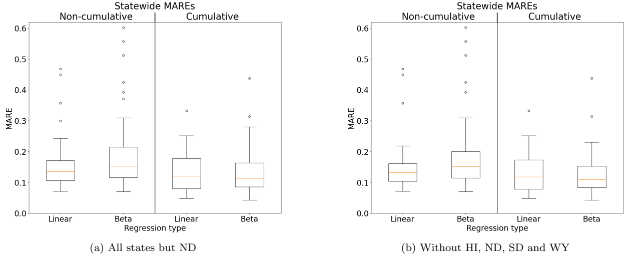
Figure 6: MARE box-plots for all states except ND, with and without the states with less than 29 rounds (HI, SD and WY).
