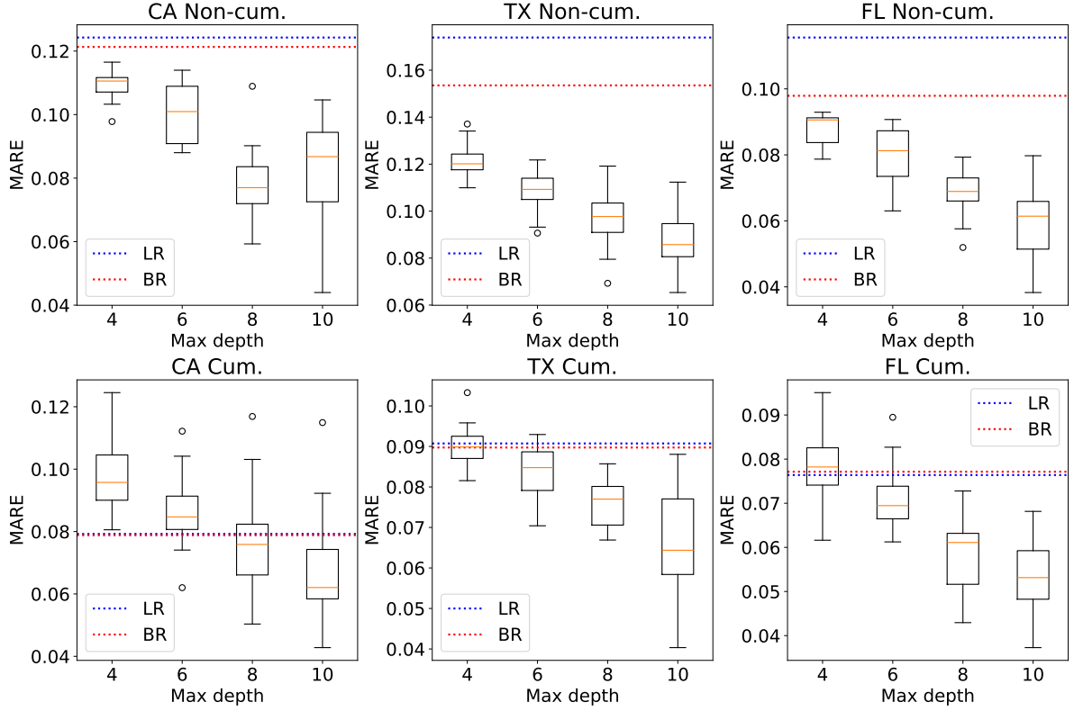
Figure 8: Box-plots of the MARE of 20 executions of the GP algorithm with different maximum depths for California (CA), Texas (TX) and Florida (FL). LR and BR MARE are shown as horizontal lines for reference.
