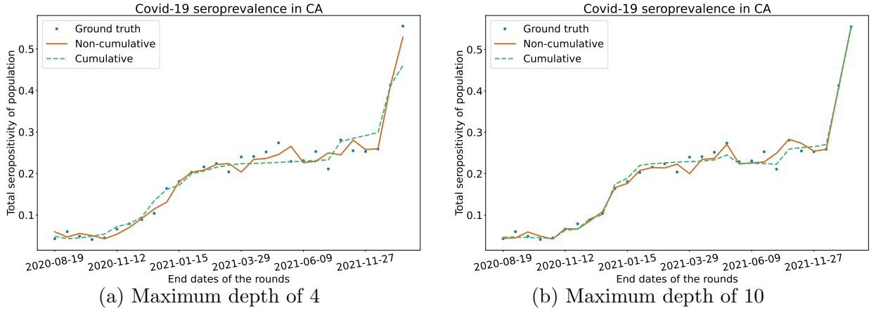
Figure 9: GP estimations of seropositivity rates for California, with a maximum depth of 4 and 10.
