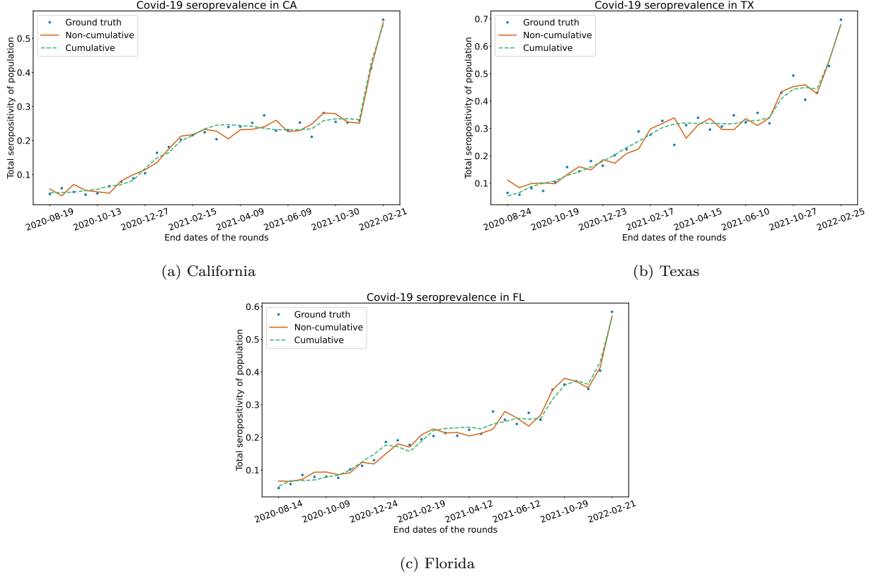
Figure 5: LR estimations of seropositivity rates for the three most populous states.
