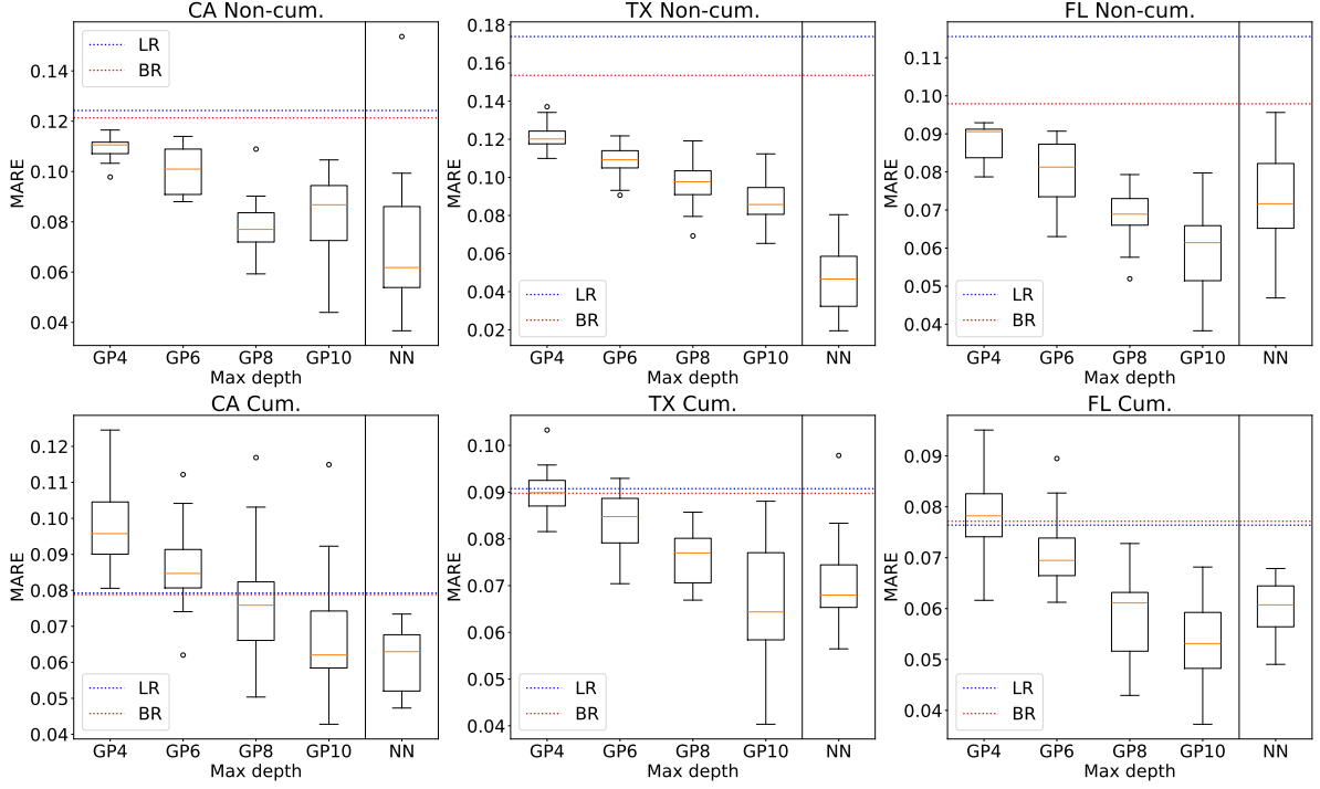
Figure 10: Box-plots of the MARE of 20 executions of the NN gradient descent algorithm for California (CA), Texas (TX) and Florida (FL). For reference, LR and BR MARE are shown as horizontal lines, and GP are shown as box-plots.
