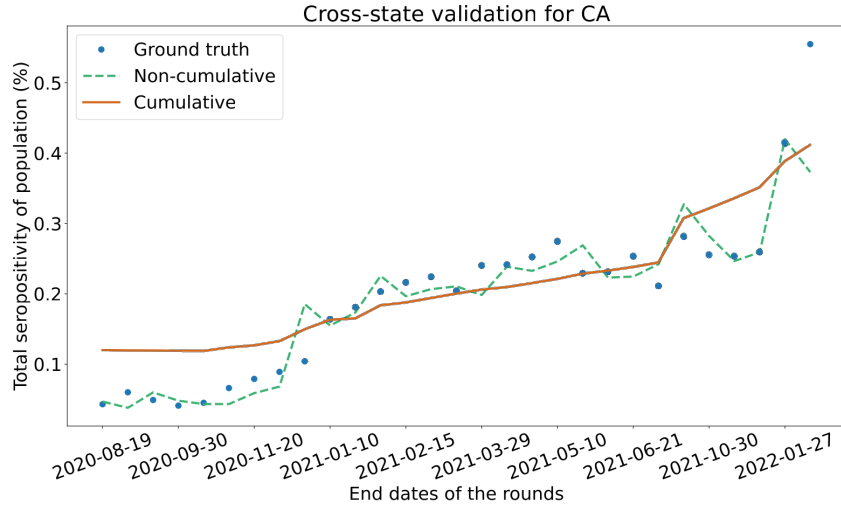
Figure 16: NN cross-state validation of California (CA) using the other ten most populous states.
