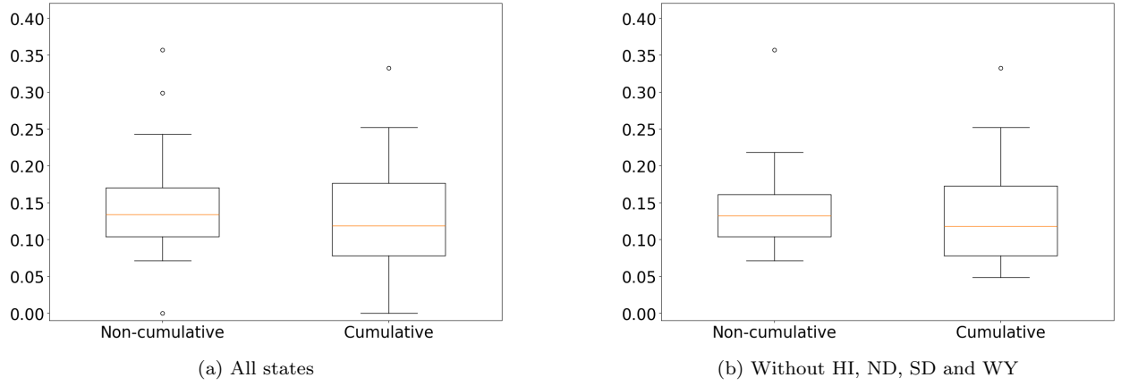
Figure 4: MARE box-plots for all states, with and without the states with less than 29 rounds (HI, ND, SD and WY), using LR.
