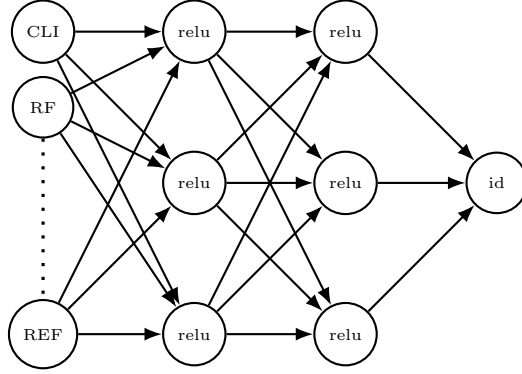
Figure 3: A simplified version of the RNN, with two hidden RELU layers, with three neurons each. The names of the input neurons represent the explanatory variables, and the names of all other neurons are their activation functions.
