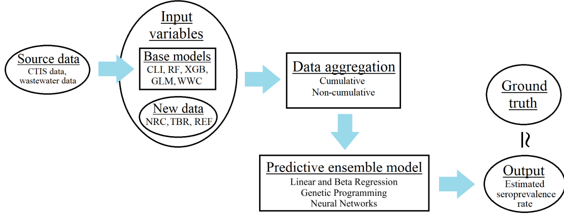
Figure 1: Diagram showing our stacking machine learning strategy. The modules are separated into two types: the circular modules represent variables or data used, and the rectangular modules represent processes performed on the data to obtain predictions (data processing and modelling). The arrows of the diagram indicate the path that the explanatory variables follow before returning an estimation of the seroprevalence rate, and then, the output is compared to the real seroprevalence using SSR and MARE as metrics.
