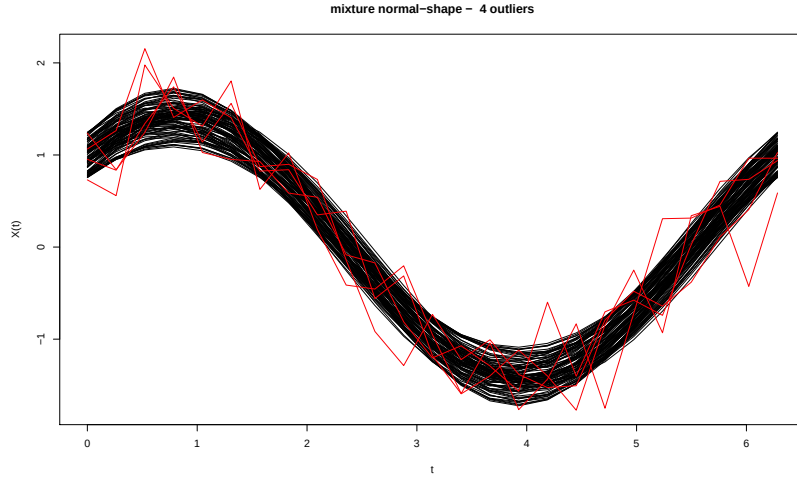
Fig. 4.E.4: Mixture model 3: shape outliers.
