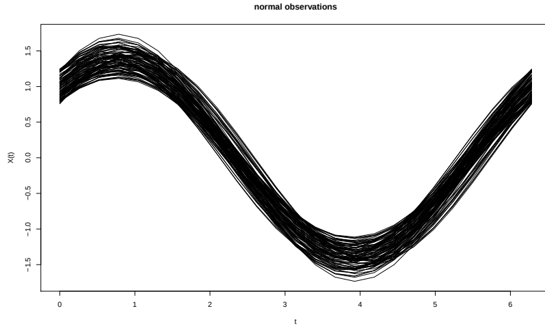
Fig. 4.E.1: Simulated observations.
