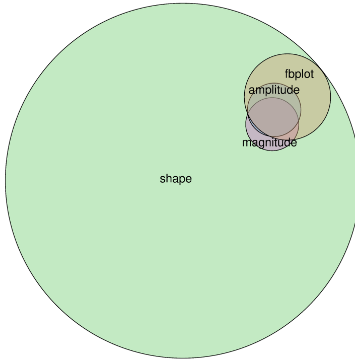
Fig. 4.3: Venn's diagram that describes the relationship between the different sets of outliers identified by MUOD (and the FBPLOT algorithm).
