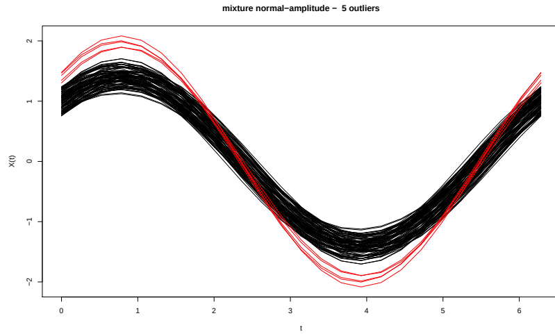
Fig. 4.E.3: Mixture model 2: amplitude outliers.
