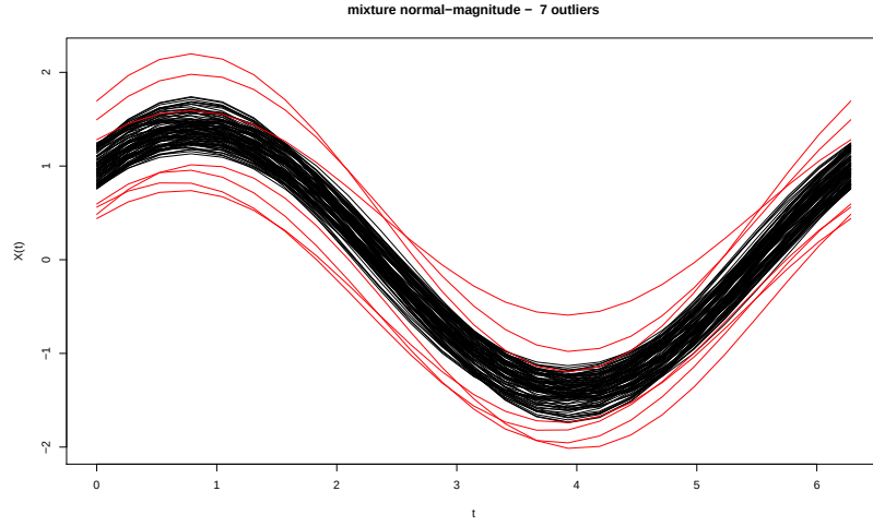
Fig. 4.E.2: Mixture model 1: magnitude outliers.
