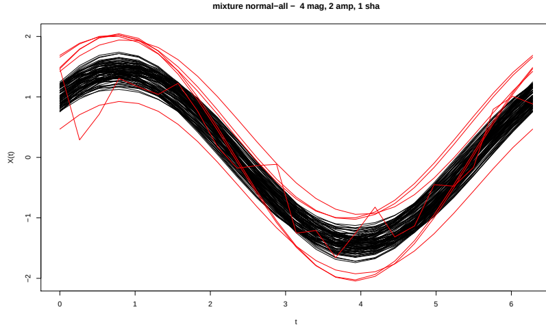
Fig. 4.E.5: Mixture model 4: magnitude, amplitude and shape outliers.
