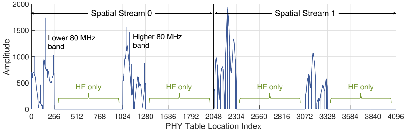
Figure 2: Layout in the PHY table of core #0 of the data associated to every OFDM subcarrier for a 160 MHz VHT frame using 2x2 MIMO. Only two spatial streams are reported here; four of them will require up to 8192 values.
