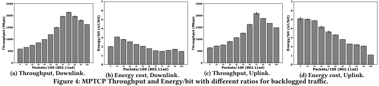
Figure 4: MPTCP Throughput and Energy/bit with different ratios for backlogged traffic.
