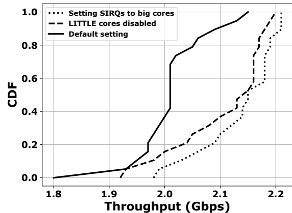
Figure 2: CDF of MPTCP throughput for various CPU settings.
