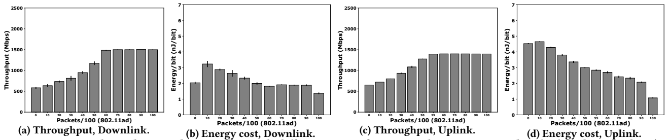
Figure 6: MPTCP Throughput and Energy/bit with different ratios for source data rate 1500 Mbps (DL) and 1400 Mbps (UL). The source data rate can be satisfied with 802.11ad alone.
