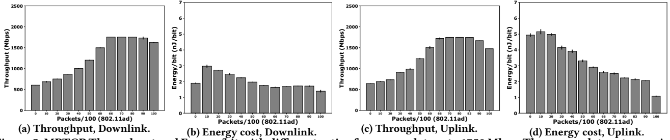
Figure 5: MPTCP Throughput and Energy/bit with different ratios for source data rate 1750 Mbps. The source data rate requires use of both interfaces.
