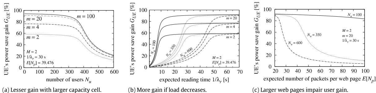
Fig. 12. Analytical evaluation of the relative power saving gain at UE.
