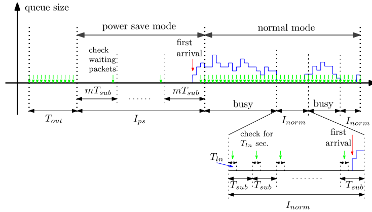
Fig. 1. Downlink queue activity with power saving and normal operation.
