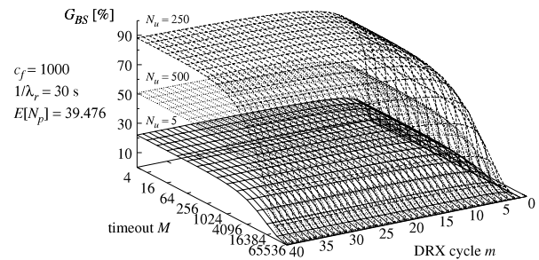
(b) Relevant gain with M \leq 1024 and m \geq 4 .
