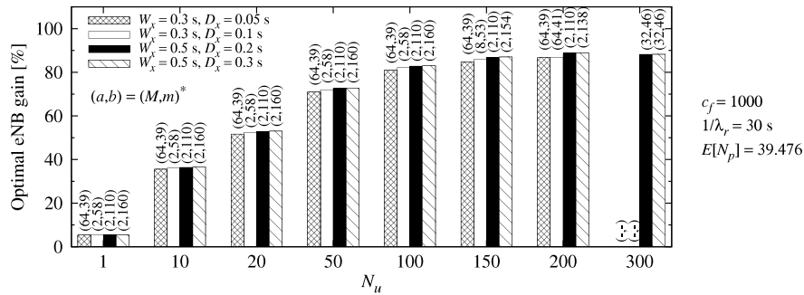
Fig. 13. Relative gain for different number of users, optimized over bounded download time and access delay.
