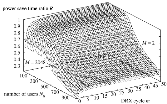
(a) Great saving opportunities with m \geq 4 .
