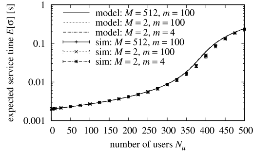
Fig. 3. E[\sigma] grows with N_u and is almost not affected by the timeout and the DRX power saving cycle durations.
