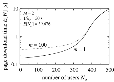
(a) E[W] grows with N_u .
