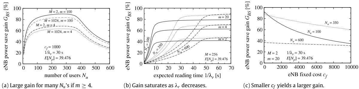
Fig. 11. G_{BS} vs. the number of cell users N_u , the reading time \frac{1}{\lambda_r} and eNB's fixed cost.
