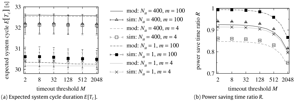
Fig. 4. Comparison of analytic and simulation results: (a) E[T_c] , and (b) R .
