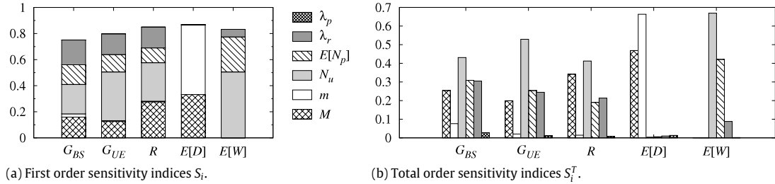
Fig. 7. Sensitivity indices of M , m , N_u , \lambda_r , \lambda_p and E[N_p] for the defined metrics.
