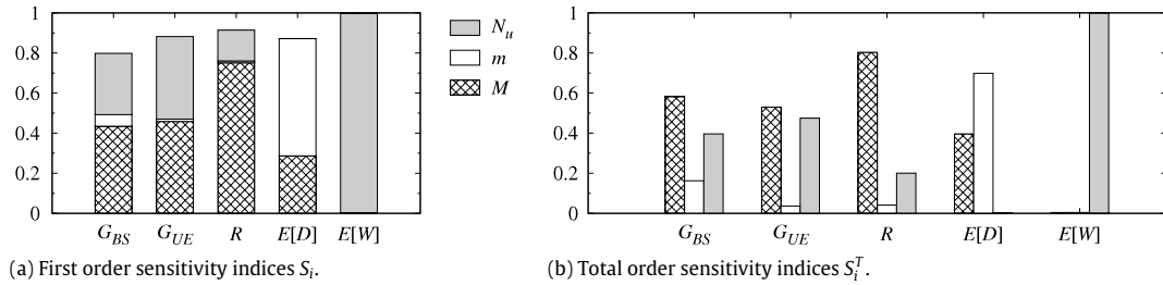
Fig. 6. Sensitivity indices of M , m and N_u for the defined metrics.
