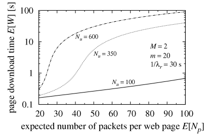
(c) E[W] increases with E[N_p] .
